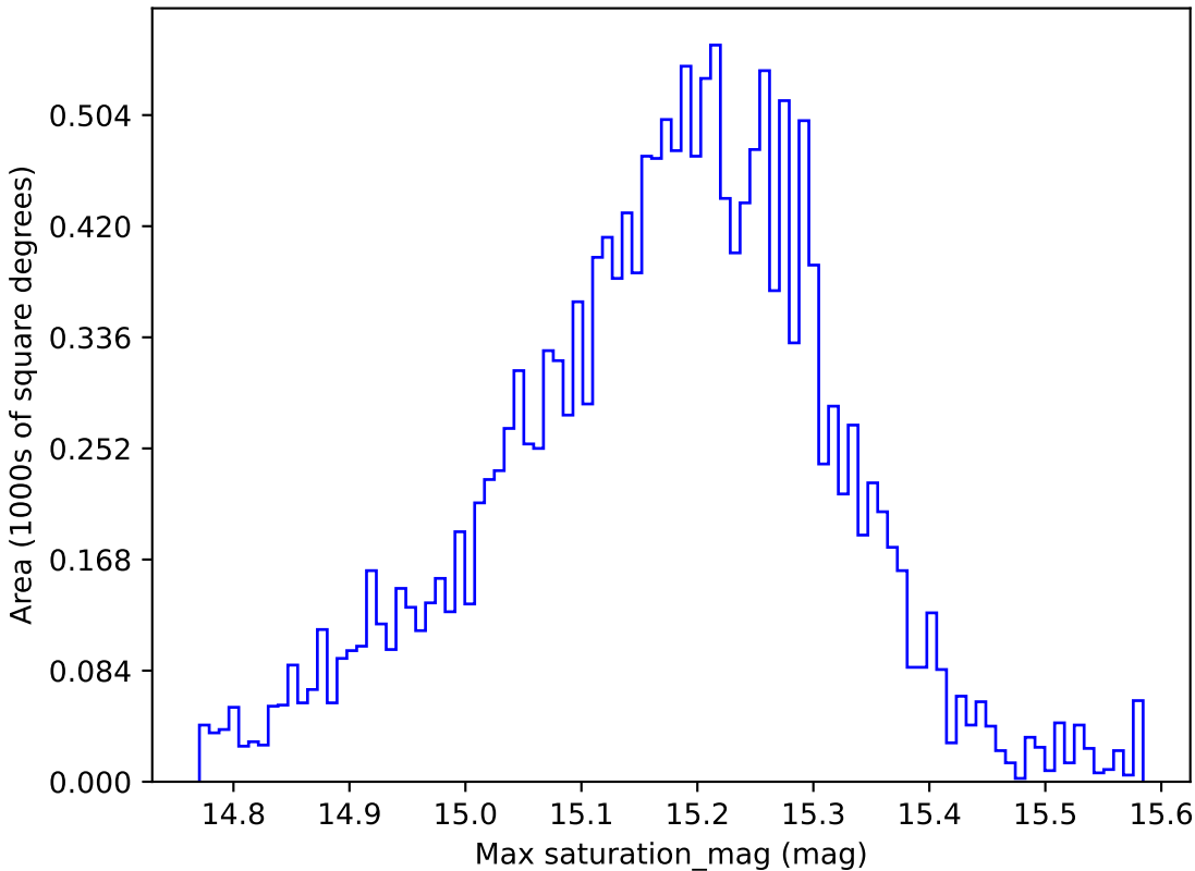
baseline_v3.5_10yrs WFD z band: Max saturation_mag
