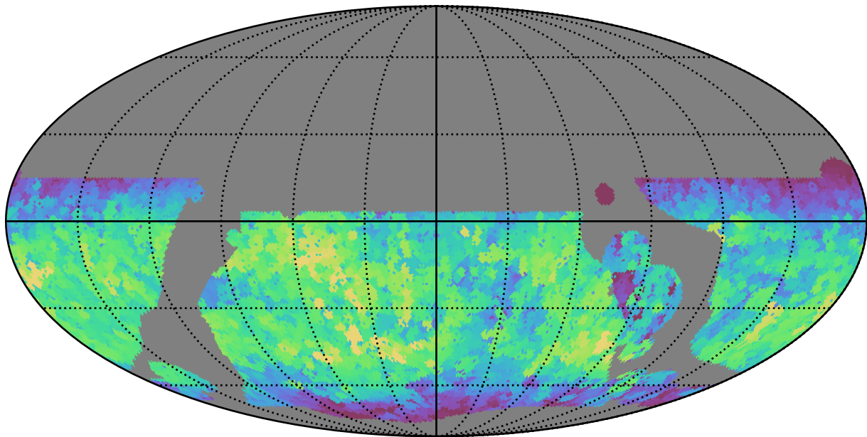
baseline_v3.5_10yrs WFD y band: Max saturation_mag
