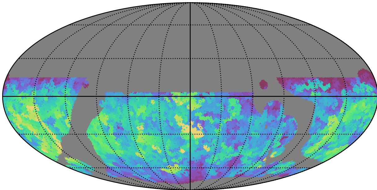
baseline_v3.5_10yrs WFD u band: Max saturation_mag
