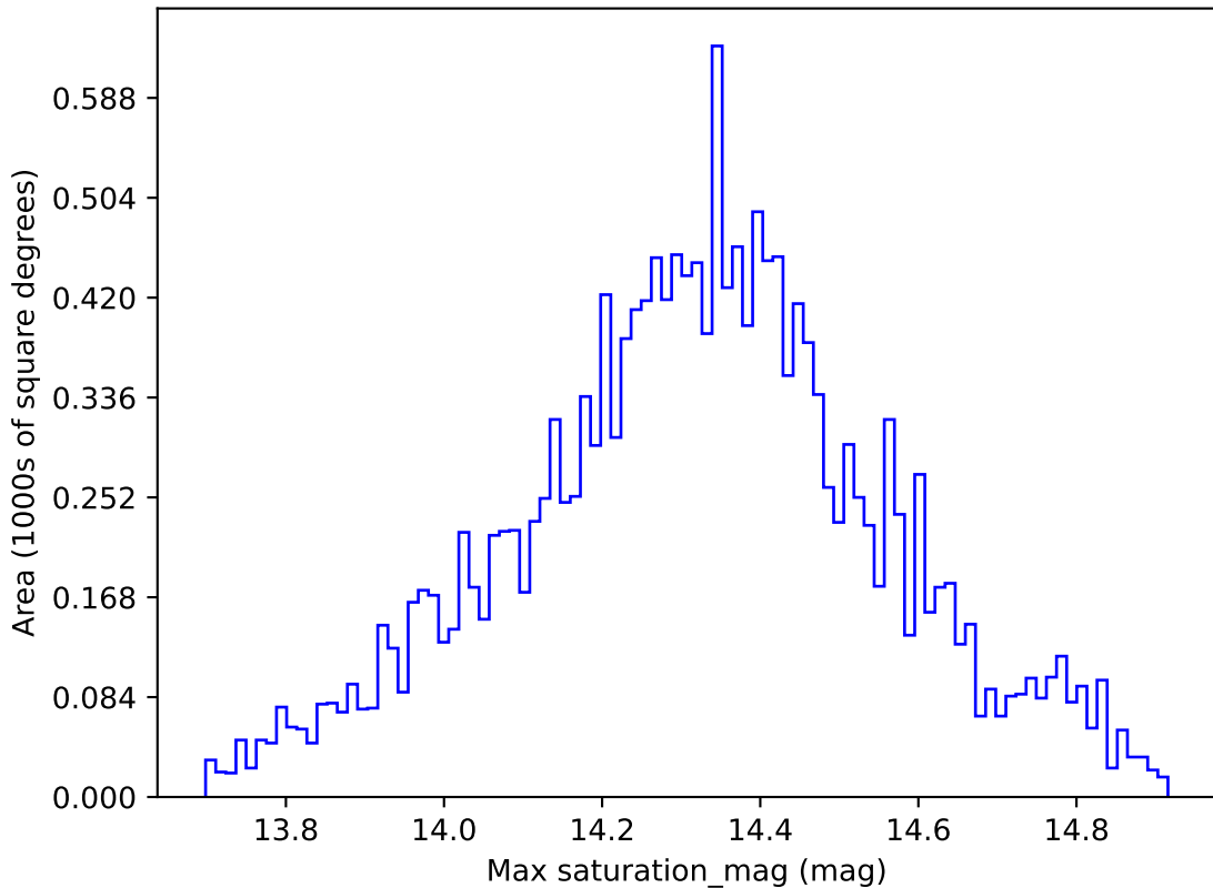
baseline_v3.5_10yrs WFD u band: Max saturation_mag
