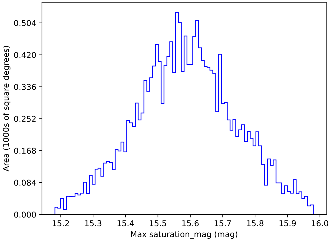
baseline_v3.5_10yrs WFD i band: Max saturation_mag
