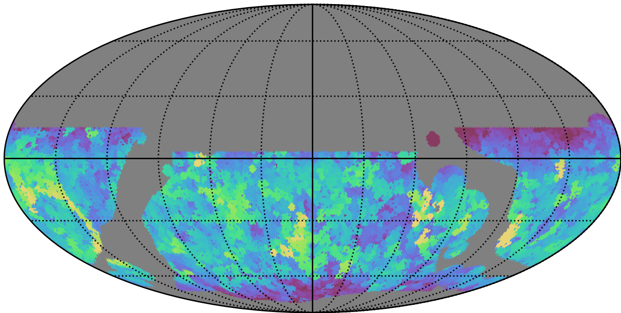
baseline_v3.5_10yrs WFD g band: Max saturation_mag
