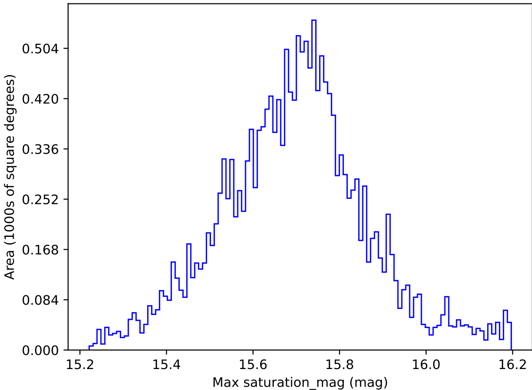
baseline_v3.5_10yrs WFD g band: Max saturation_mag
