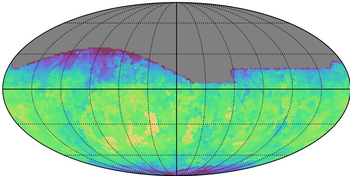
baseline_v3.5_10yrs All sky z band: Max saturation_mag
