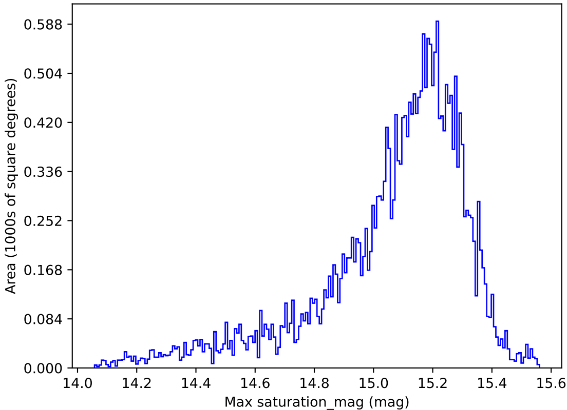
baseline_v3.5_10yrs All sky z band: Max saturation_mag
