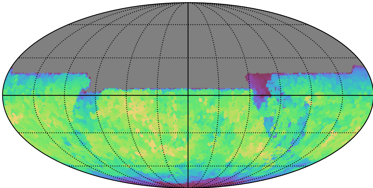
baseline_v3.5_10yrs All sky y band: Max saturation_mag
