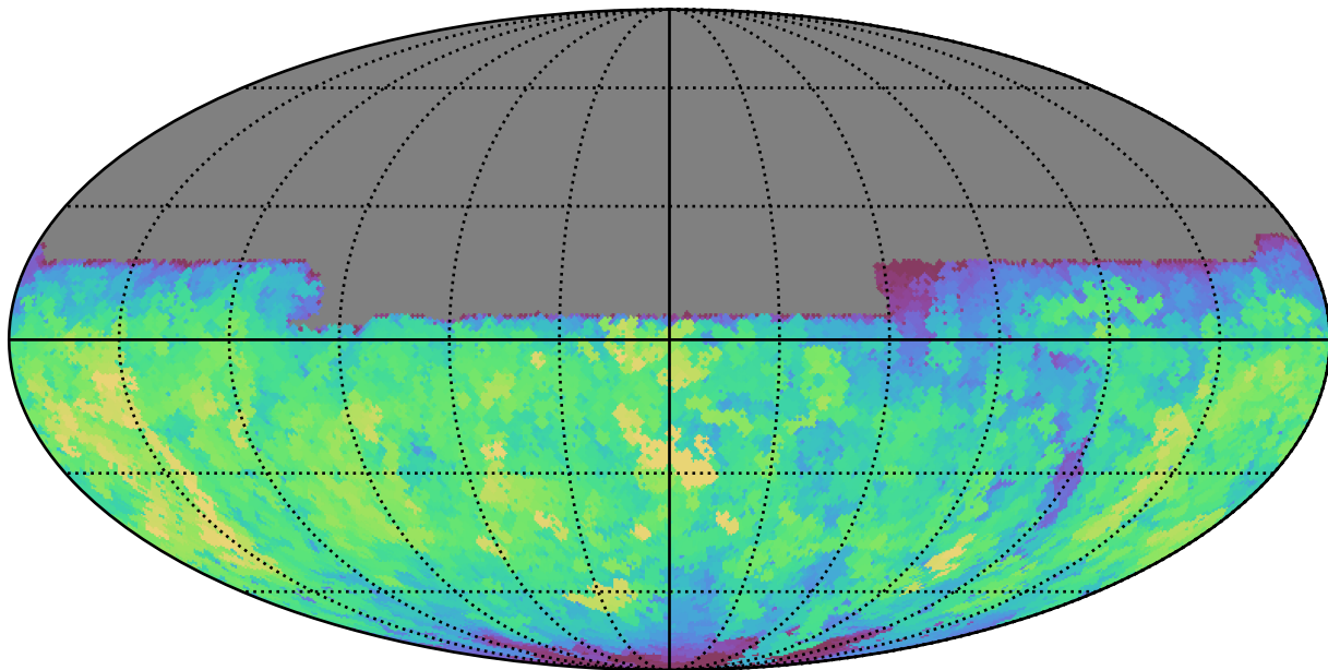
baseline_v3.5_10yrs All sky u band: Max saturation_mag
