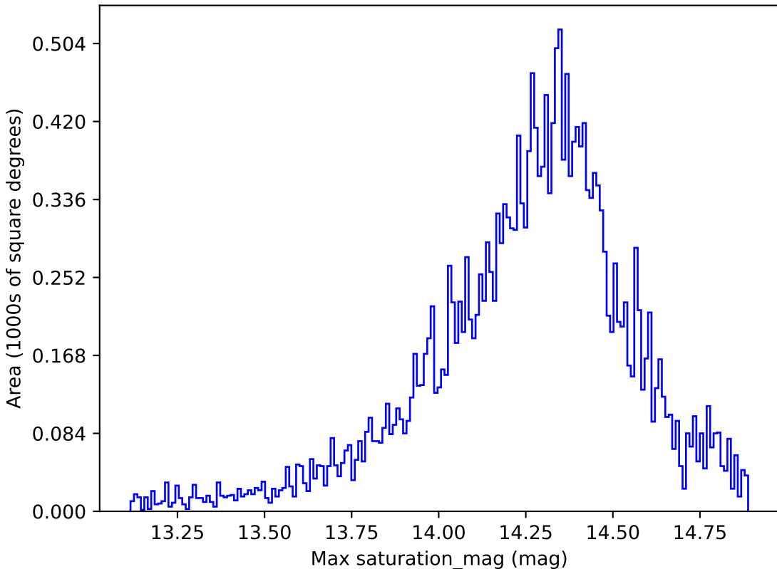
baseline_v3.5_10yrs All sky u band: Max saturation_mag
