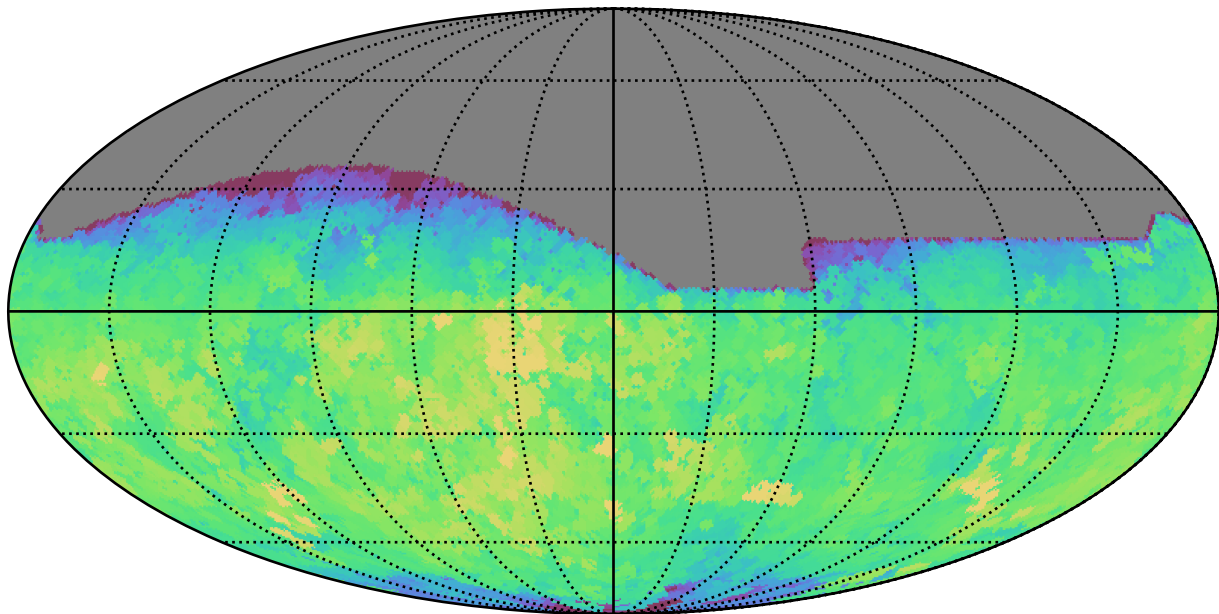
baseline_v3.5_10yrs All sky r band: Max saturation_mag
