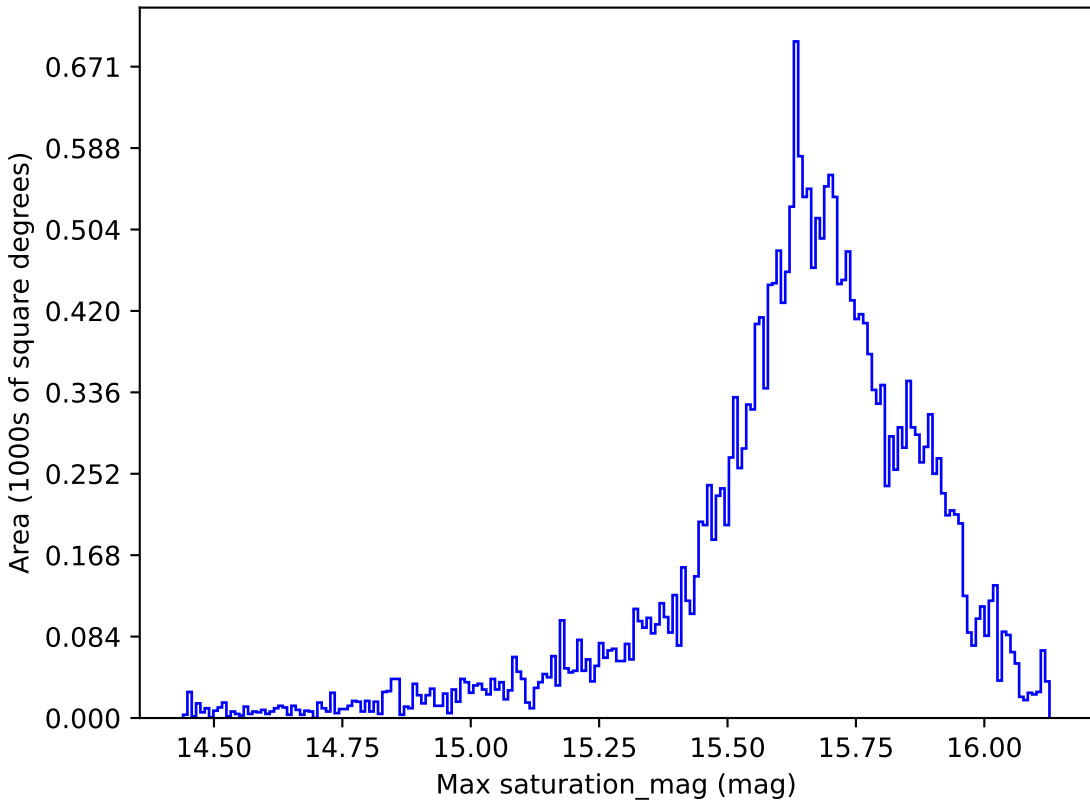
baseline_v3.5_10yrs All sky r band: Max saturation_mag
