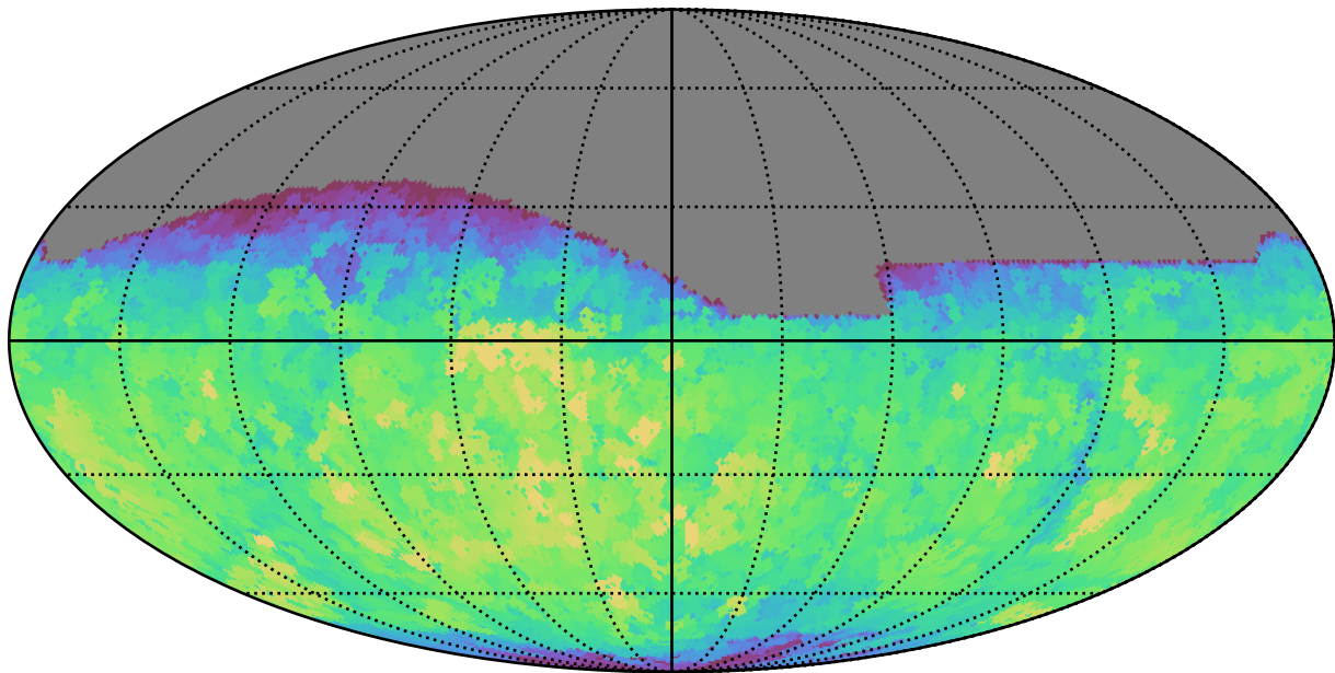
baseline_v3.5_10yrs All sky i band: Max saturation_mag
