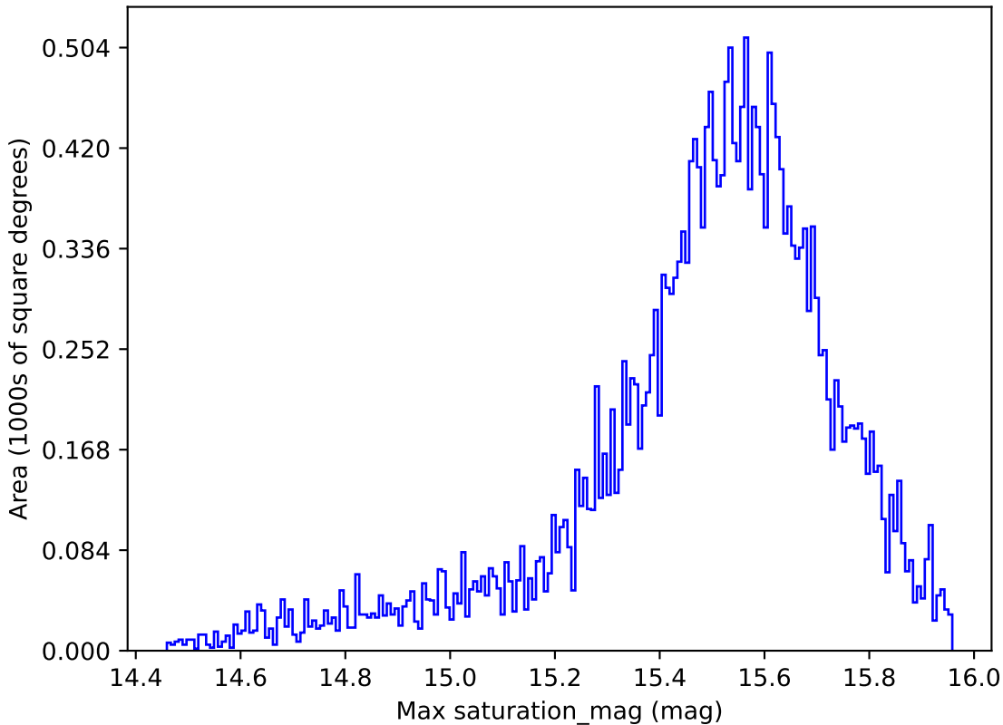
baseline_v3.5_10yrs All sky i band: Max saturation_mag
