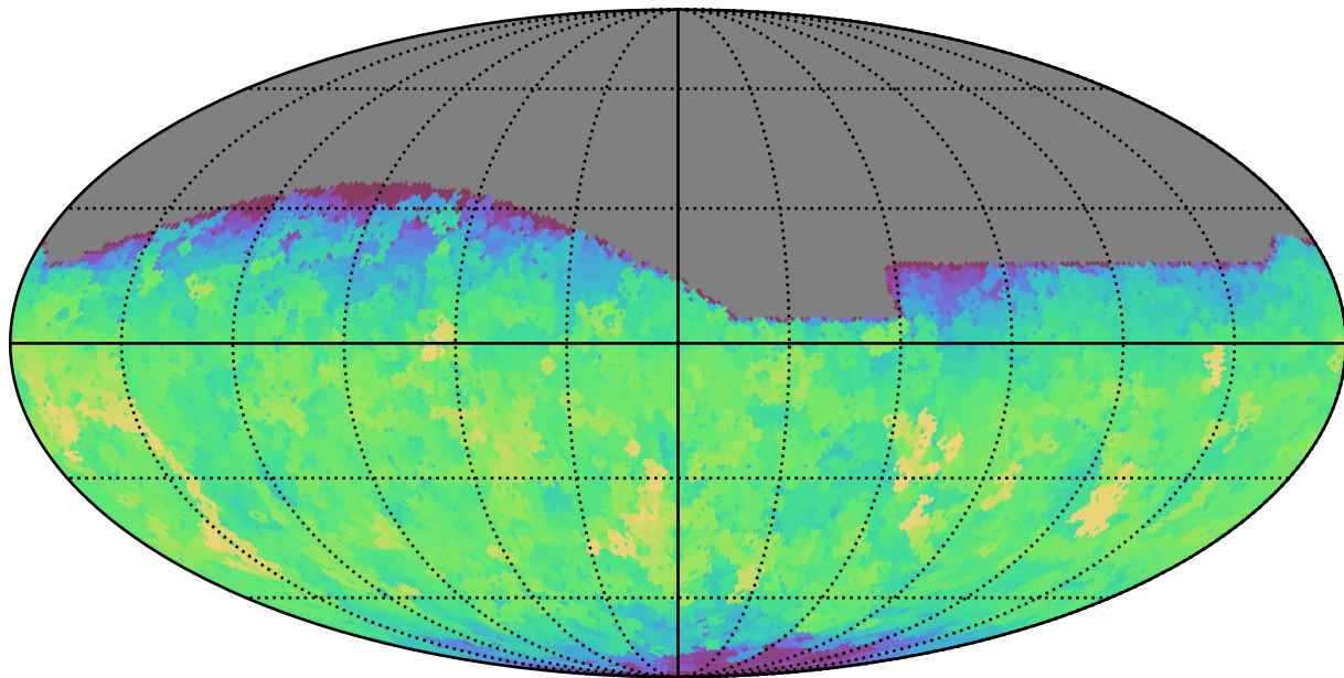
baseline_v3.5_10yrs All sky g band: Max saturation_mag
