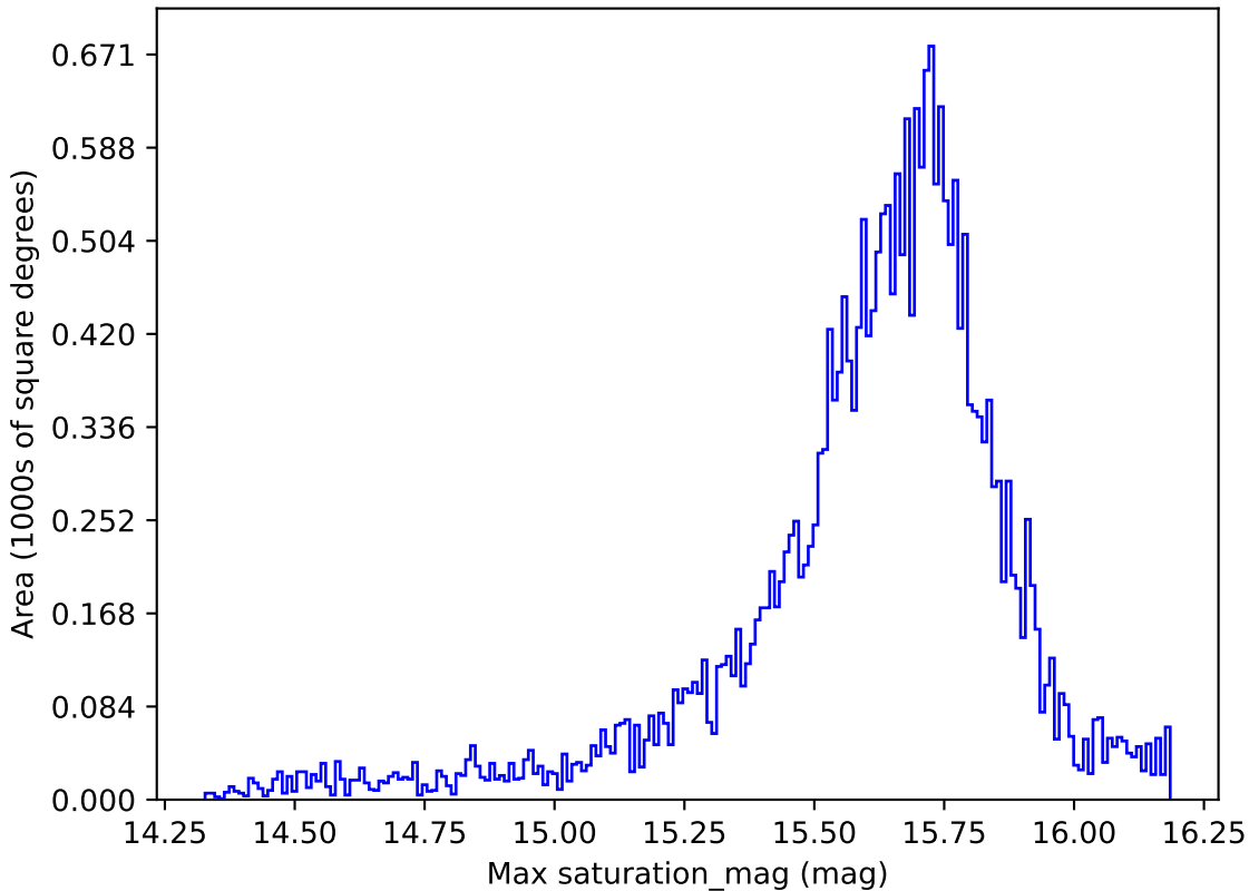
baseline_v3.5_10yrs All sky g band: Max saturation_mag
