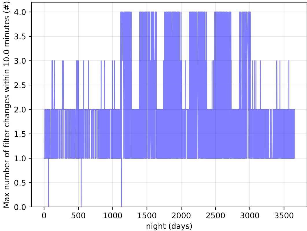
baseline_v3.5_10yrs Per Night: Max number of filter changes within 10.0 minutes
