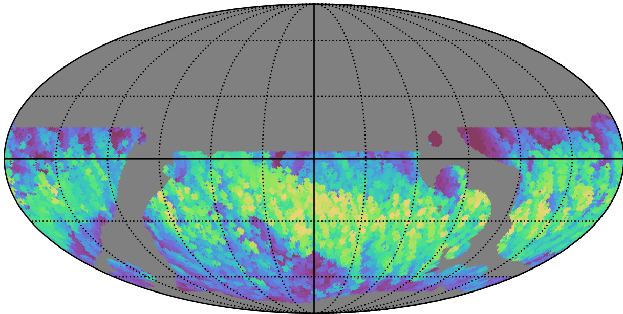
baseline_v3.5_10yrs WFD z band: Max normairmass
