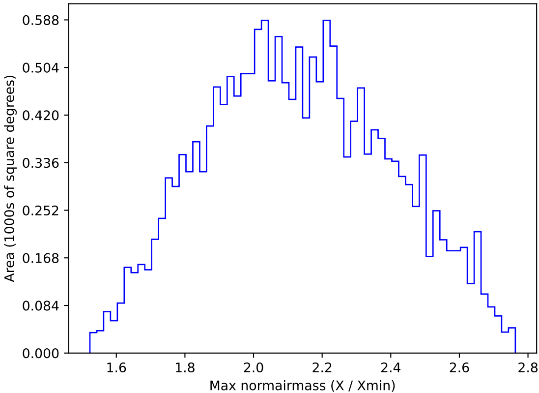
baseline_v3.5_10yrs WFD y band: Max normairmass
