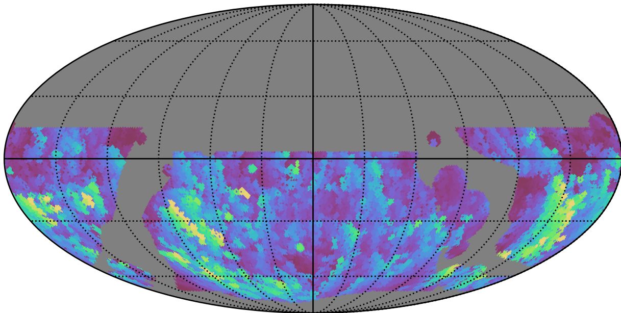
baseline_v3.5_10yrs WFD u band: Max normairmass
