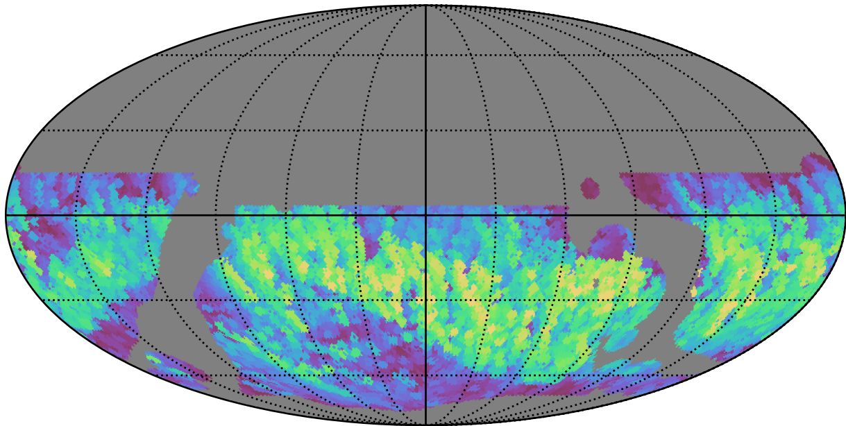
baseline_v3.5_10yrs WFD r band: Max normairmass
