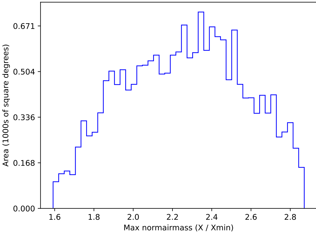
baseline_v3.5_10yrs WFD i band: Max normairmass
