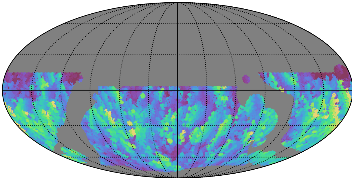
baseline_v3.5_10yrs WFD g band: Max normairmass
