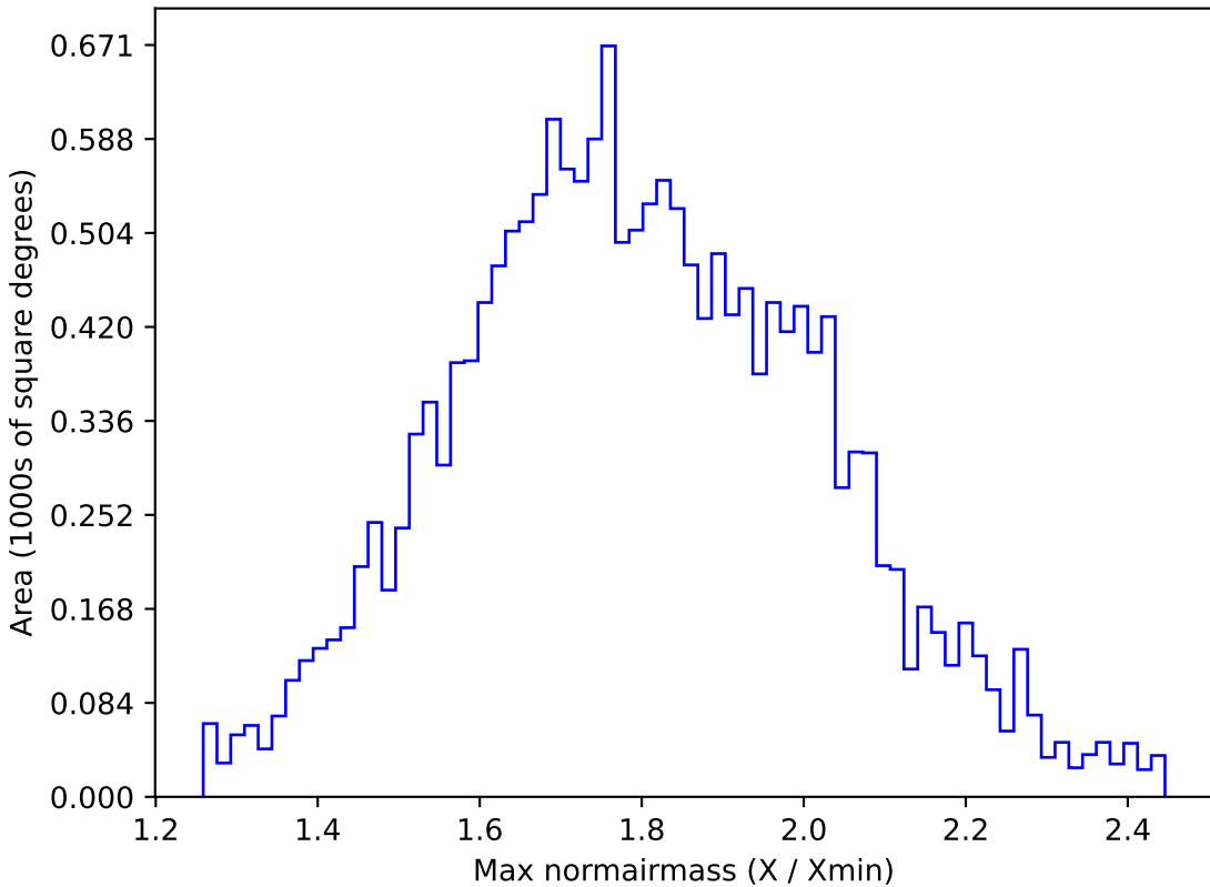
baseline_v3.5_10yrs WFD g band: Max normairmass
