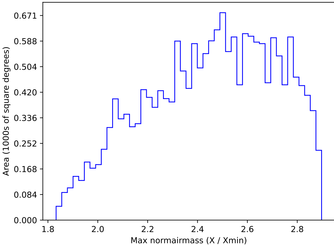
baseline_v3.5_10yrs WFD all bands: Max normairmass
