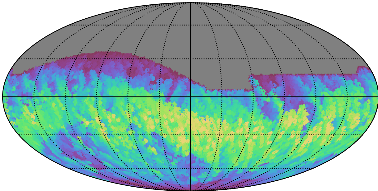
baseline_v3.5_10yrs All sky z band: Max normairmass
