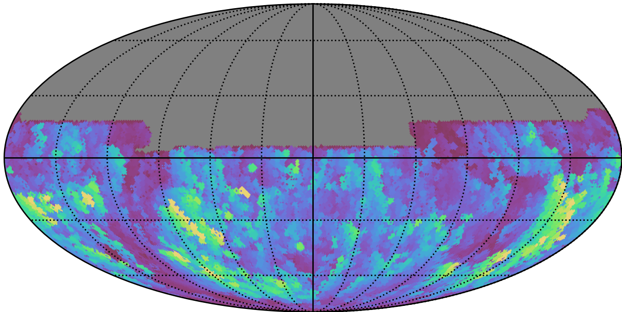
baseline_v3.5_10yrs All sky u band: Max normairmass
