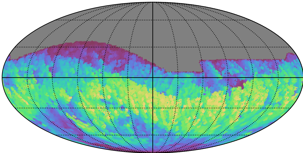
baseline_v3.5_10yrs All sky i band: Max normairmass
