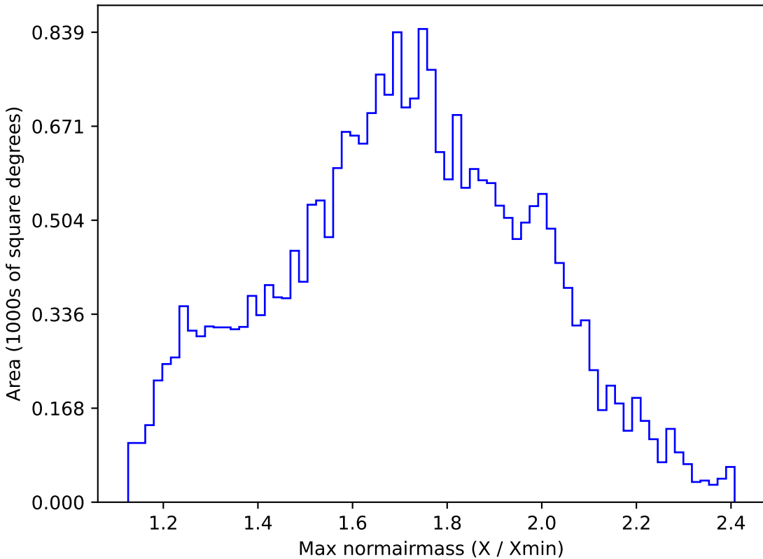
baseline_v3.5_10yrs All sky g band: Max normairmass
