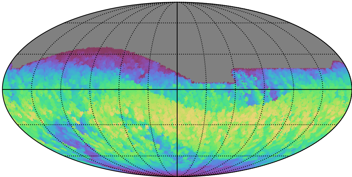
baseline_v3.5_10yrs All sky all bands: Max normairmass
