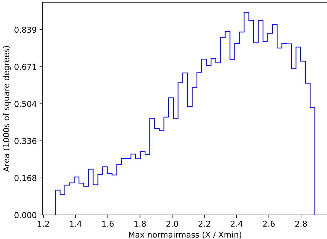
baseline_v3.5_10yrs All sky all bands: Max normairmass
