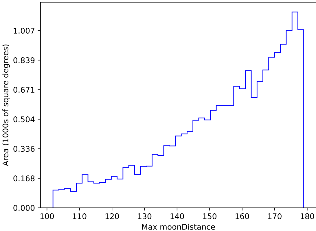
baseline_v3.5_10yrs WFD z band: Max moonDistance
