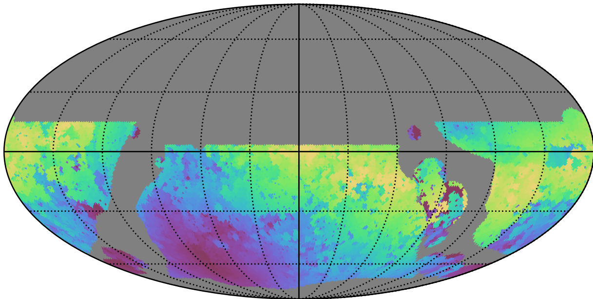
baseline_v3.5_10yrs WFD y band: Max moonDistance
