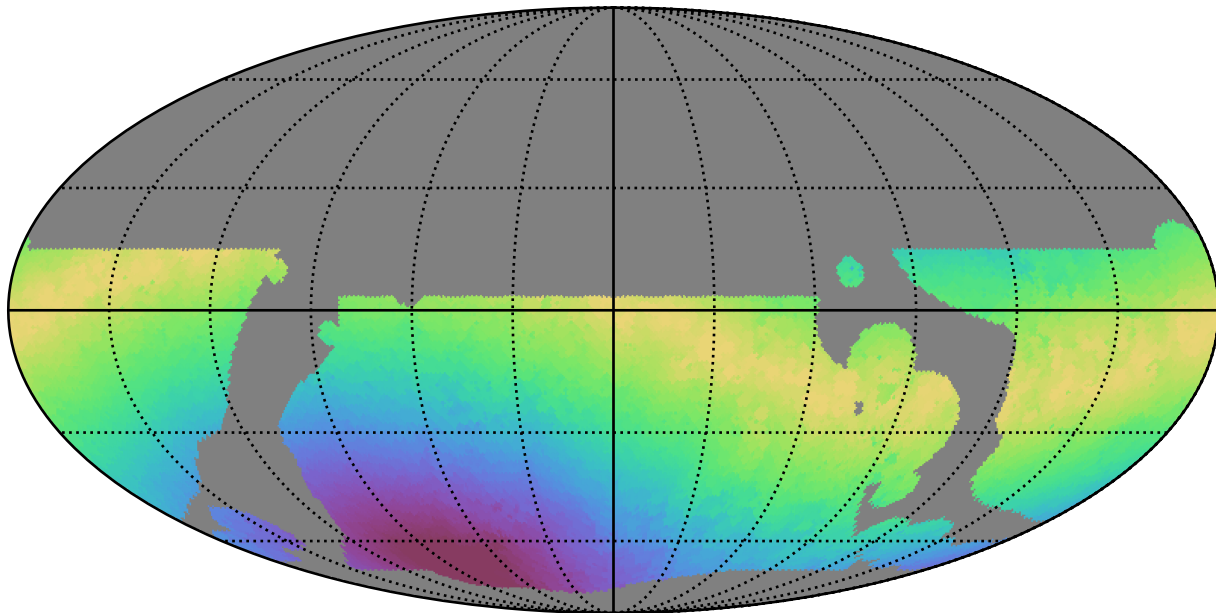
baseline_v3.5_10yrs WFD u band: Max moonDistance
