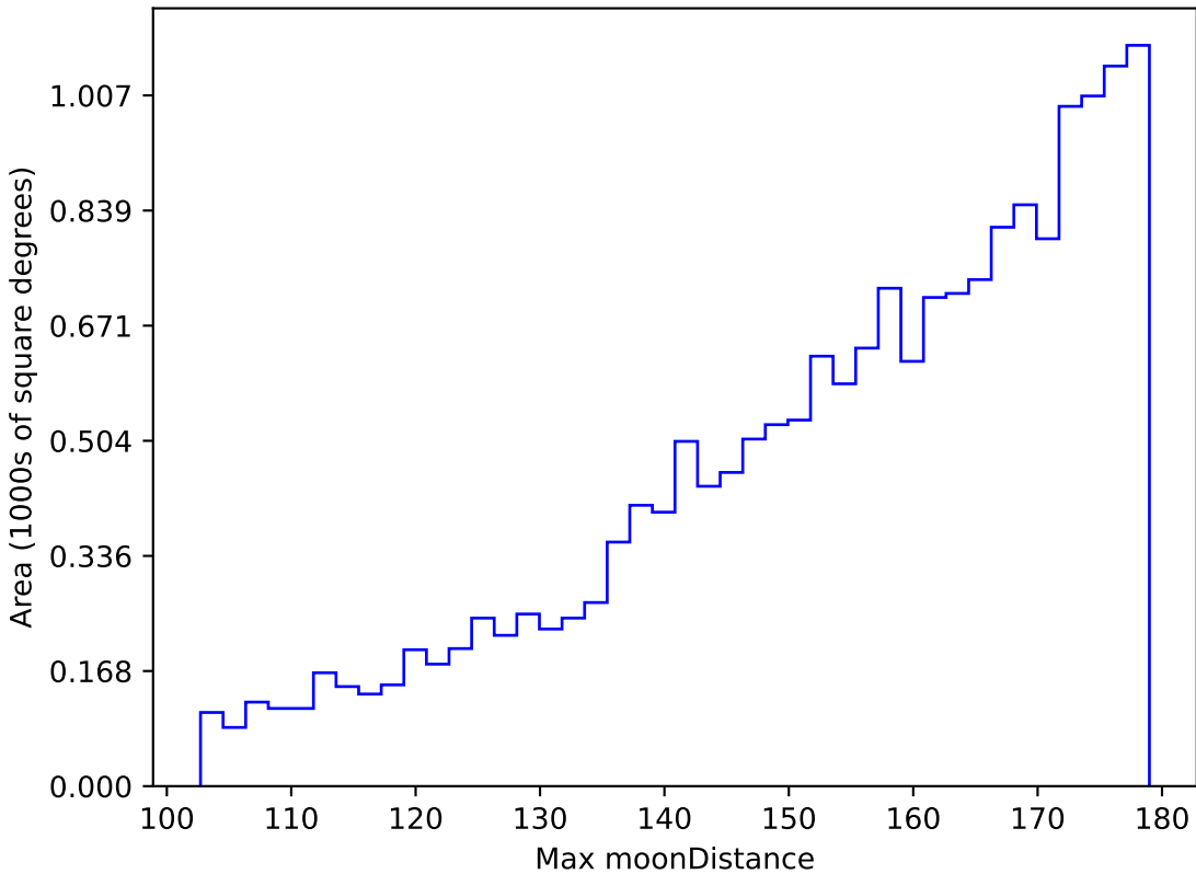
baseline_v3.5_10yrs WFD u band: Max moonDistance
