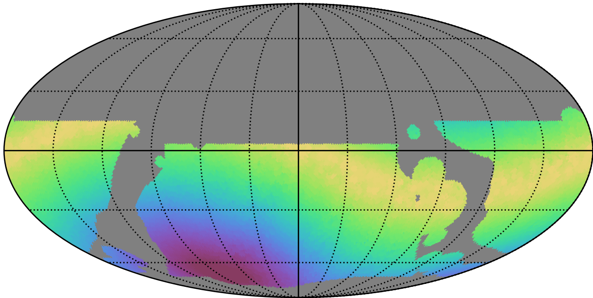
baseline_v3.5_10yrs WFD r band: Max moonDistance
