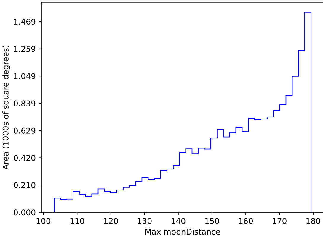
baseline_v3.5_10yrs WFD r band: Max moonDistance
