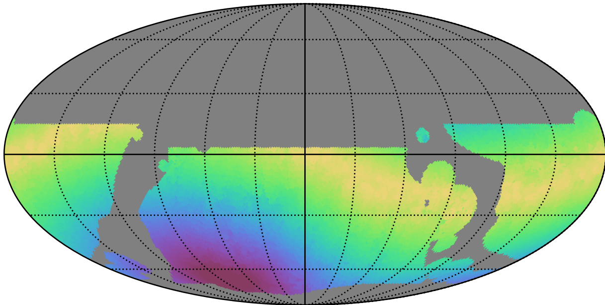
baseline_v3.5_10yrs WFD i band: Max moonDistance
