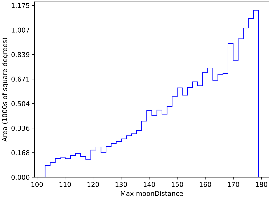
baseline_v3.5_10yrs WFD g band: Max moonDistance
