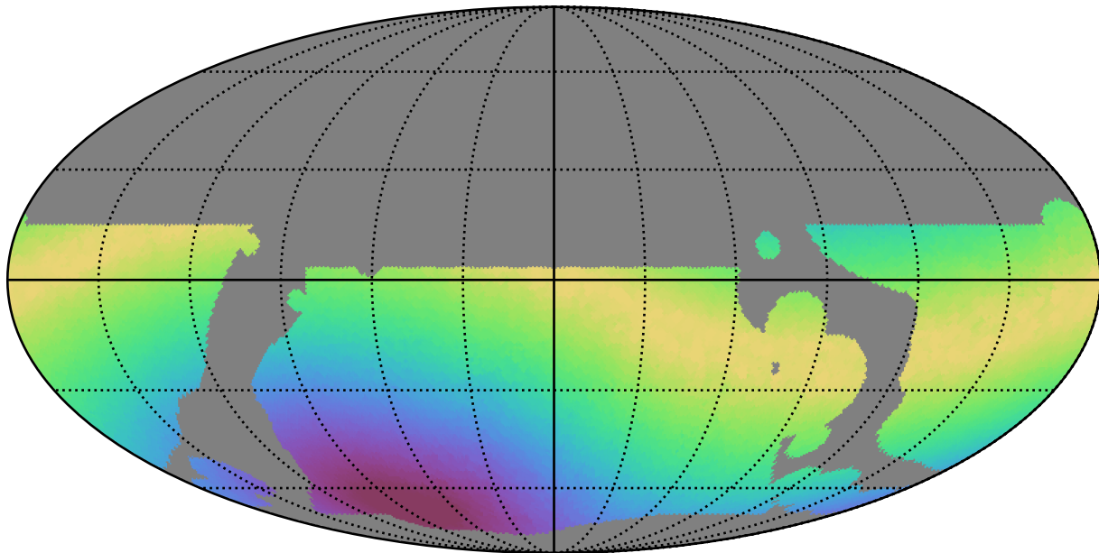
baseline_v3.5_10yrs WFD all bands: Max moonDistance
