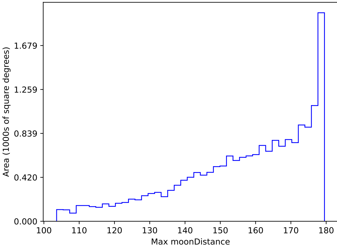
baseline_v3.5_10yrs WFD all bands: Max moonDistance
