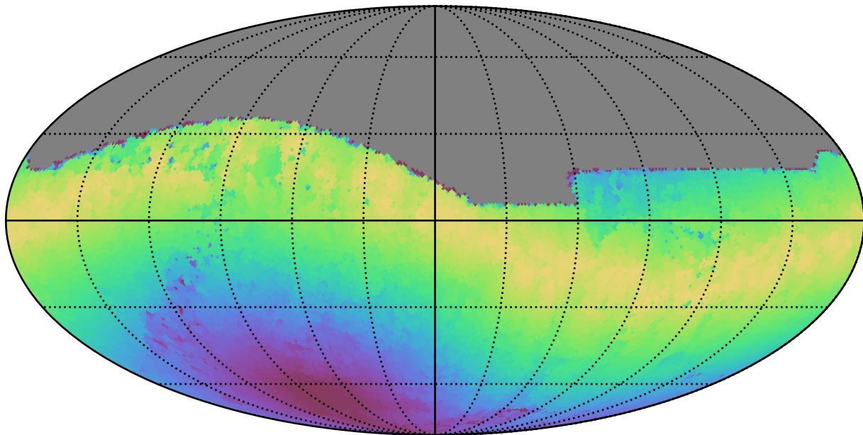
baseline_v3.5_10yrs All sky z band: Max moonDistance
