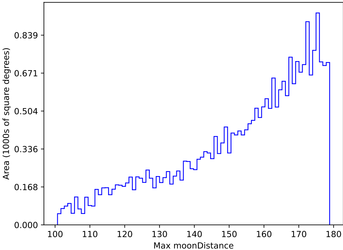
baseline_v3.5_10yrs All sky z band: Max moonDistance
