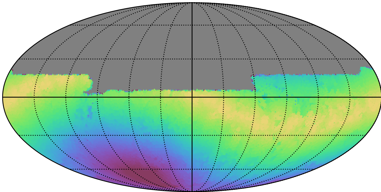
baseline_v3.5_10yrs All sky u band: Max moonDistance
