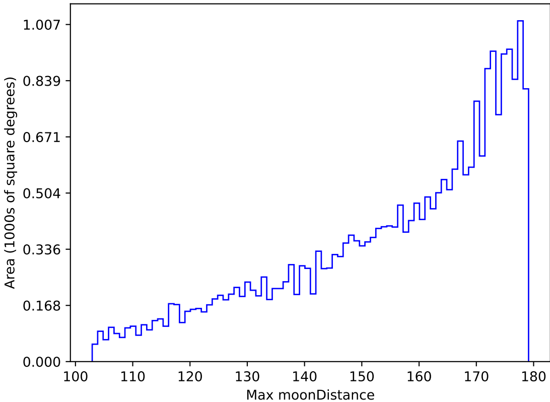
baseline_v3.5_10yrs All sky i band: Max moonDistance
