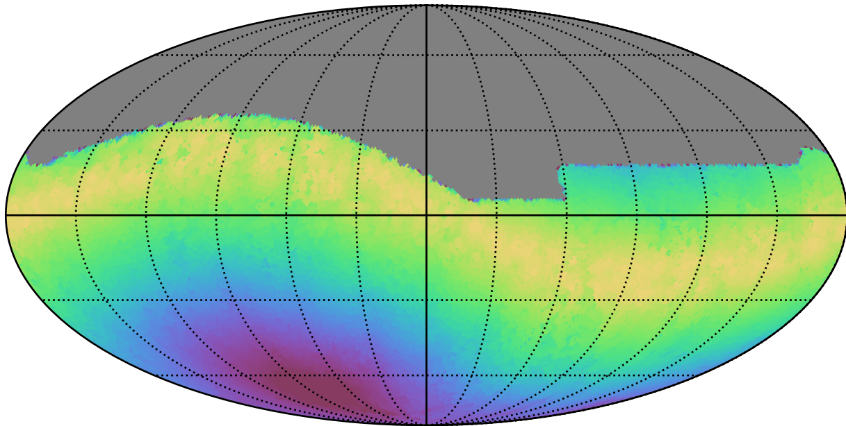
baseline_v3.5_10yrs All sky g band: Max moonDistance
