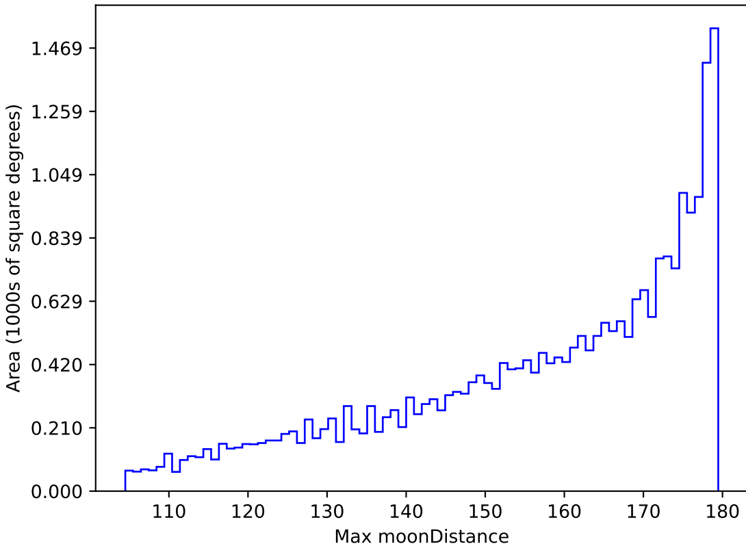
baseline_v3.5_10yrs All sky all bands: Max moonDistance
