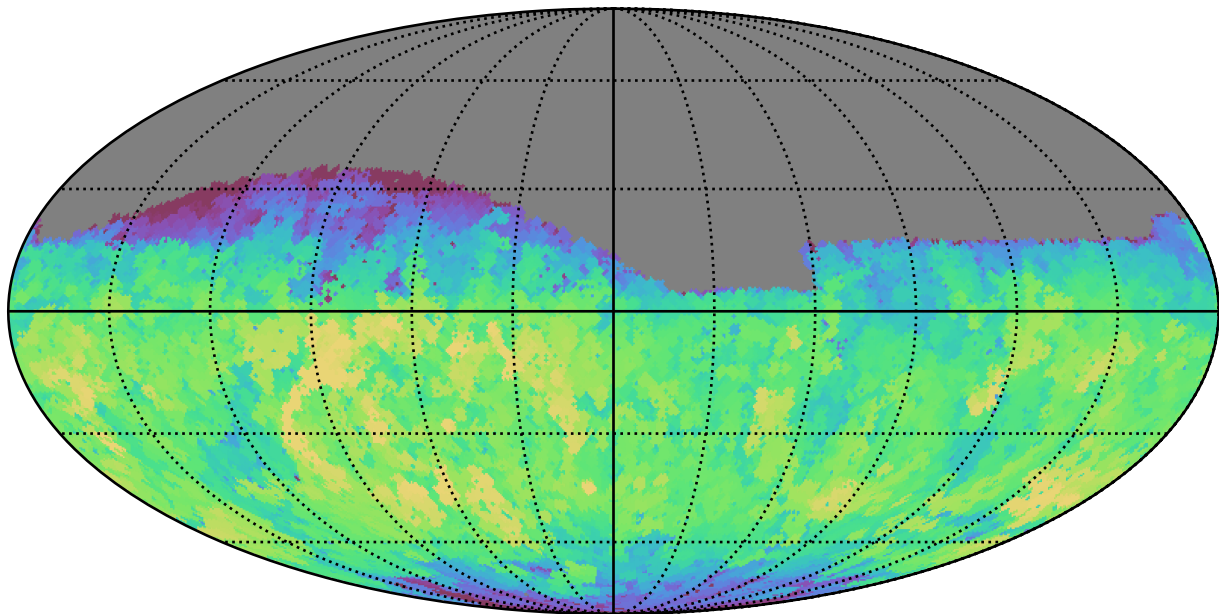
baseline_v3.5_10yrs Yr 1 z band: Max fiveSigmaDepth
